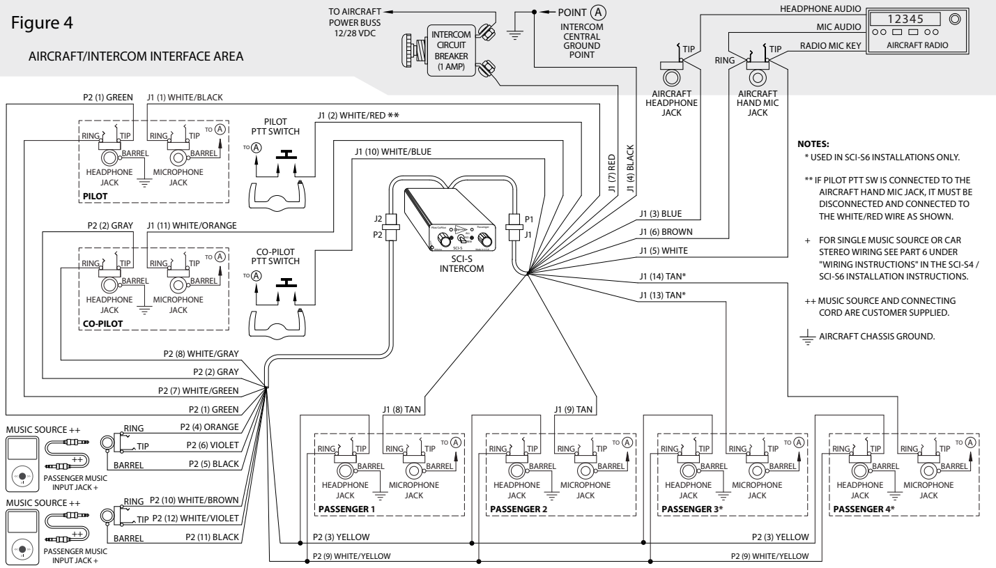
SCI-S4 / SCI-S6 INSTALLATION WIRING DIAGRAM
